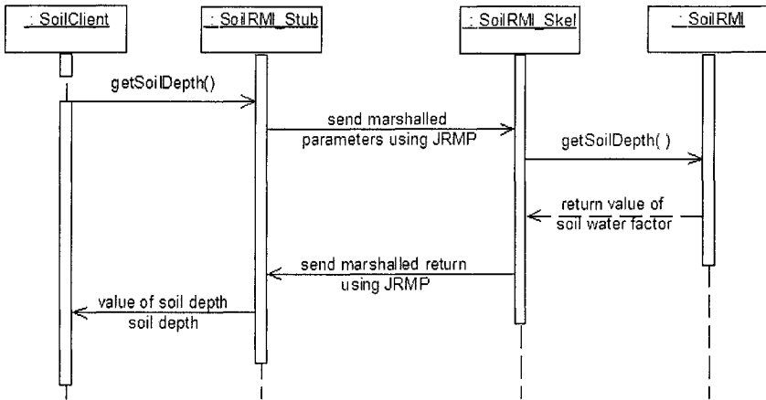
Figure 11-13. Collaboration between client and server objects using RMI.
