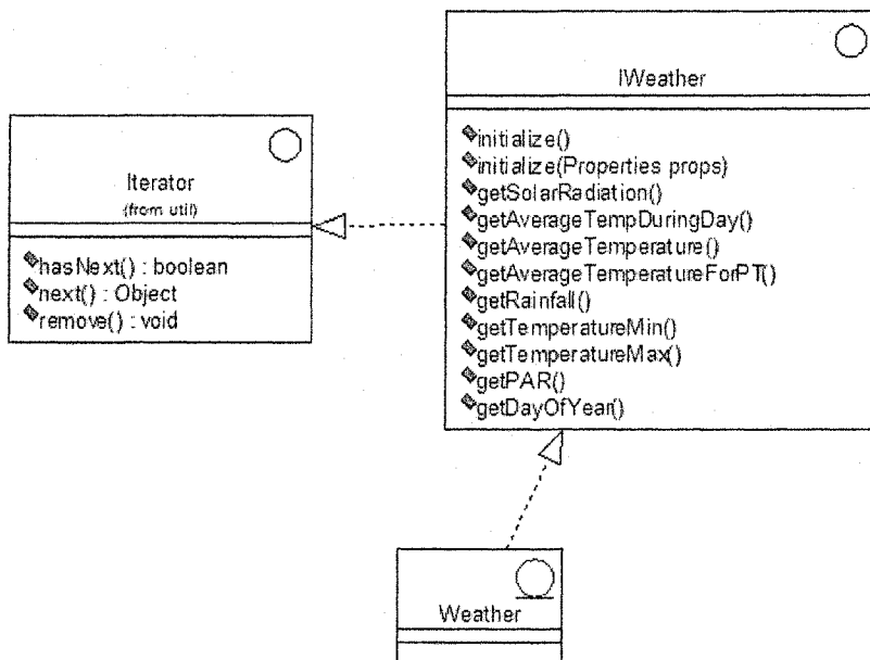
Figure 8-33. Class Weather implements the behavior defined in IWeather and Iterator.
