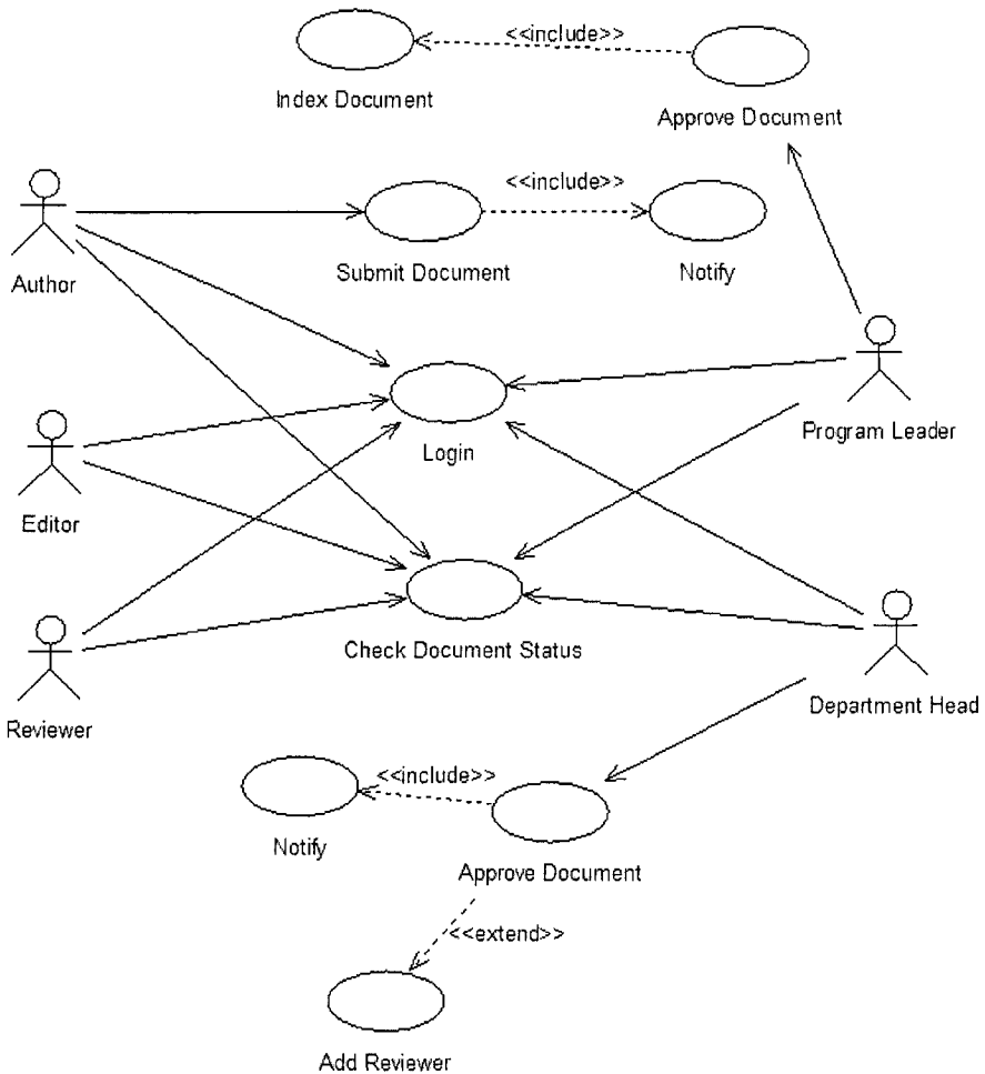
Figure 6-1. The use case model for a document tracking system.
