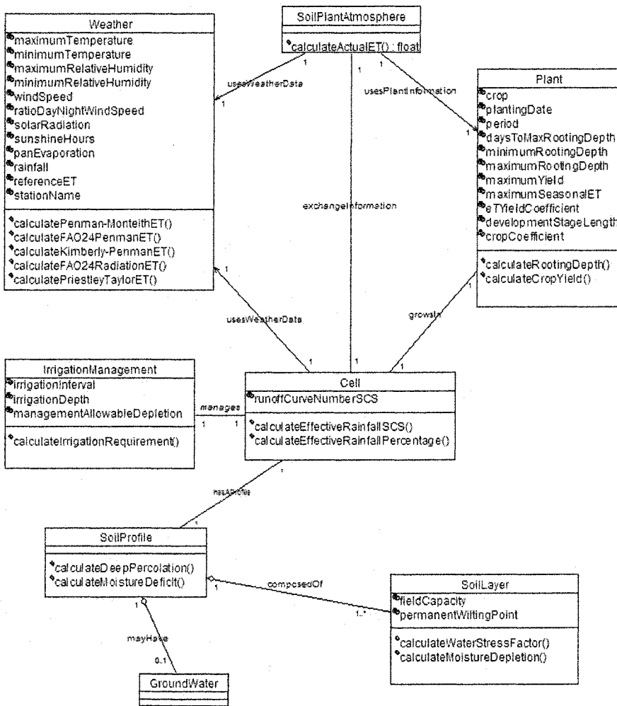
Figure 10-6. Class diagram for the ISM model.
