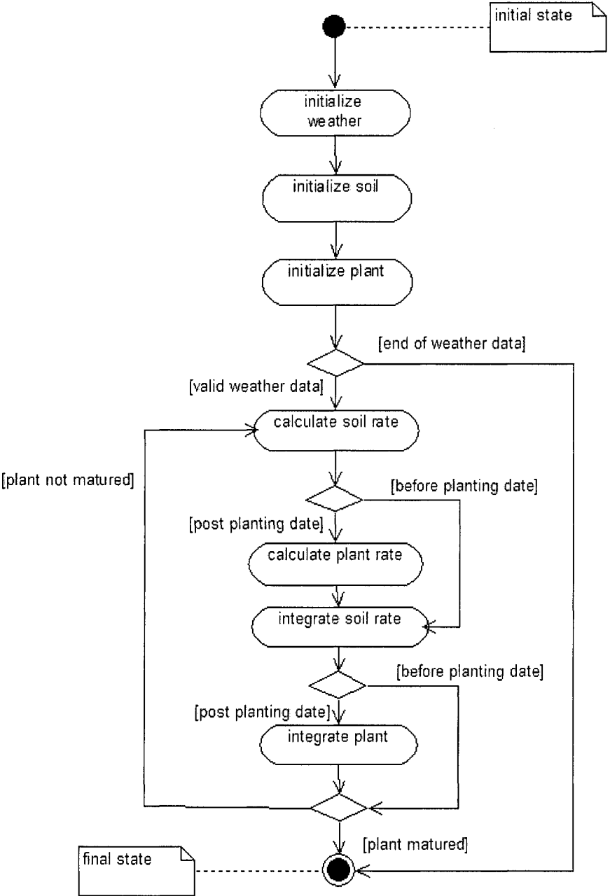
Figure 6-10. Example of an activity diagram.
