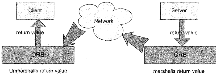
Figure 11-5. ORB sends back to client the answer from server.
