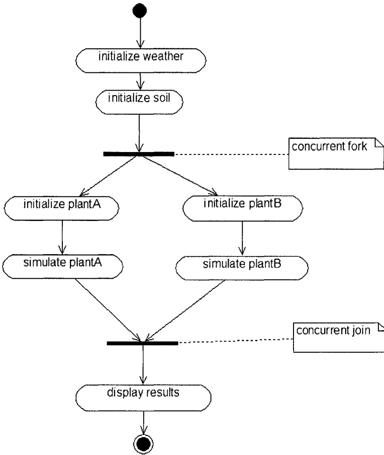
Figure 6-11. Example of concurrent processing of activities.
