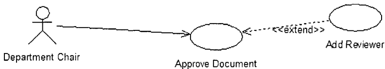
Figure 5-6. Use case Add Reviewer extends base use case Approve Document.
