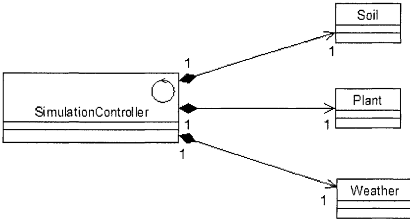
Figure 8-18. Relationship between control and entity classes.
