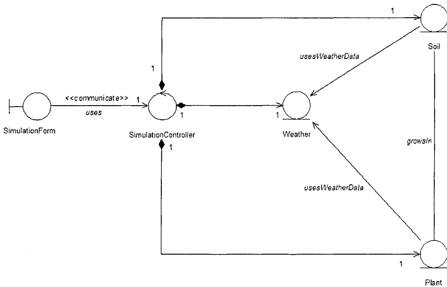
Figure 8-19. Class diagram for the Kraalingen simulation approach.
