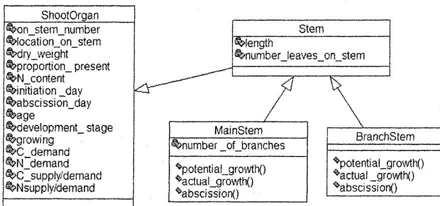
Figure 4-17. Example of a hierarchy of classes related by inheritance.
