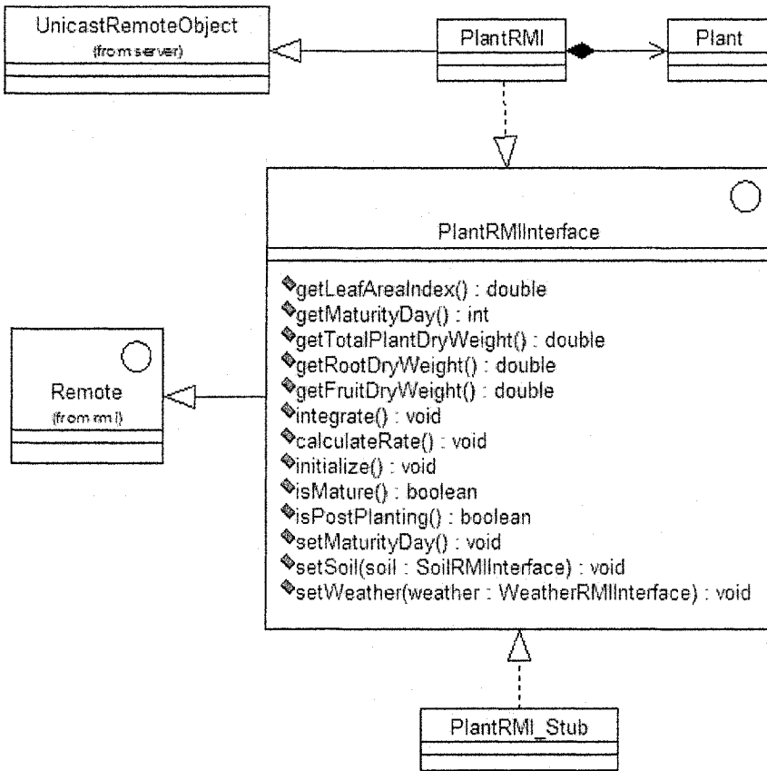
Figure 11-19. Links between objects and interfaces for remote communication.
