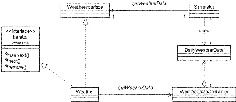
Figure 7-17. Another class diagram for Iterator.
