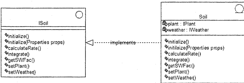
Figure 8-31. Class Soil implements ISoil interface.
