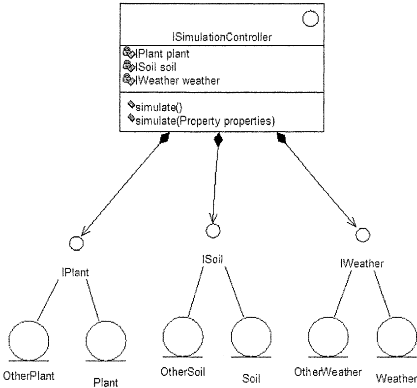
Figure 8-24. Interfaces allow for plugging in other class/components.
