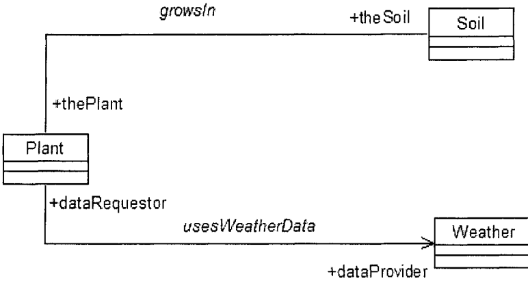
Figure 4-6. Example of class Plant playing different roles in different associations.
