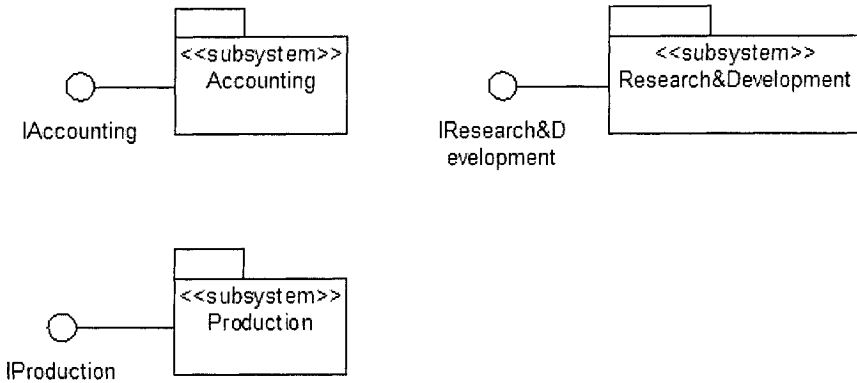
Figure 3-13. Decomposition of a system into subsystems.
