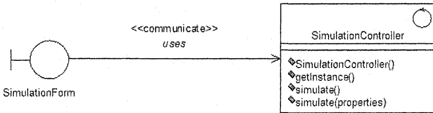
Figure 8-17. A boundary object communicating with a control object.
