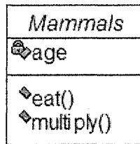
Figure 4-21. Example of an abstract class. The name of the class is written in italics.
