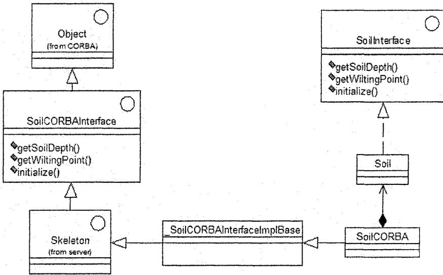
Figure 11-6. Class diagram for SoilCORBAServer.
