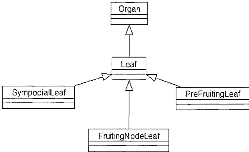
Figure 4-18. Hierarchy of classes in a cotton simulation model.
