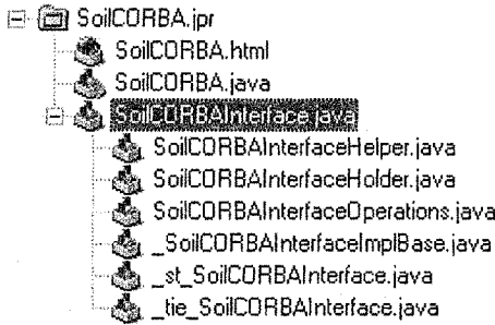
Figure 11-8. Files created by CORBA's IDL compiler.
