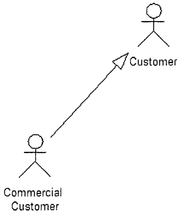
Figure 5-2. Actors related using a generalization relationship.
