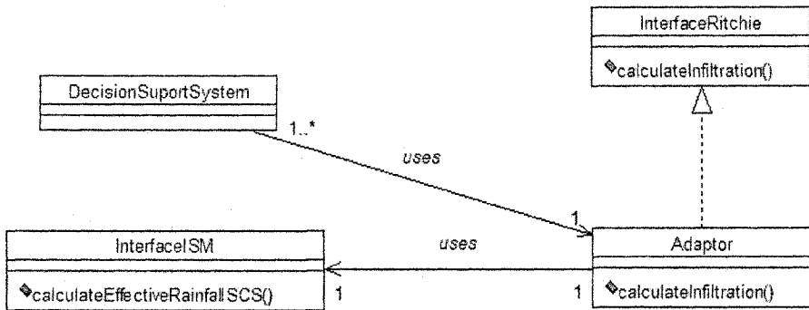
Figure 7-10. An adaptor allows communication between classes that do not implement the same interface.
