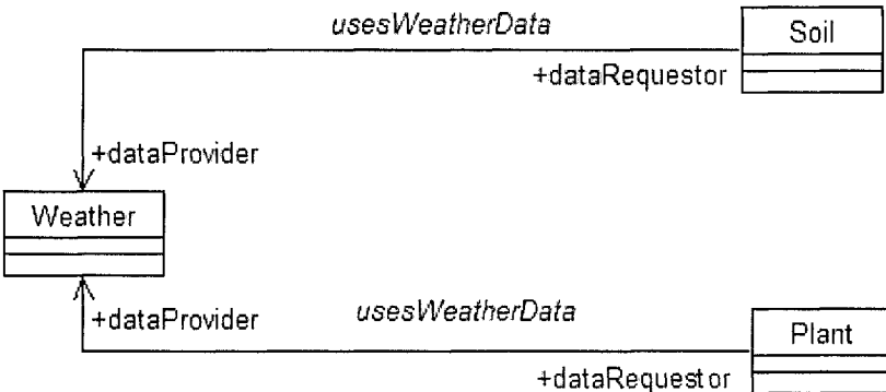
Figure 4-7. Class Weather plays the same role in two different associations.
