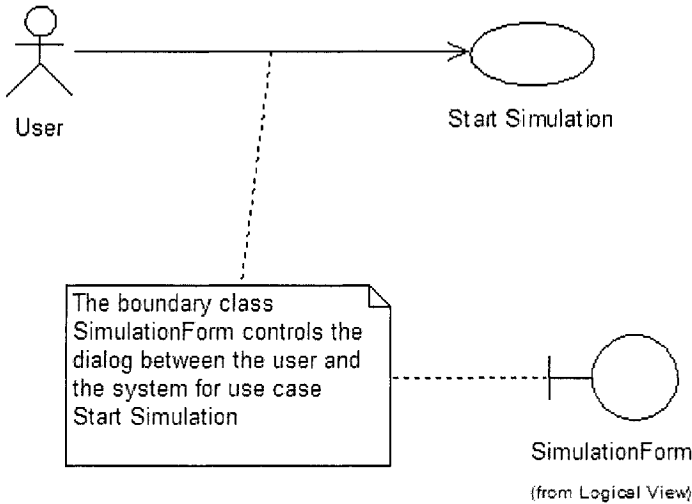
Figure 8-11. One boundary class controls the dialog between an actor and a use case.
