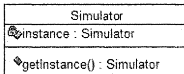
Figure 7-7. Example of implementation of the singleton pattern.
