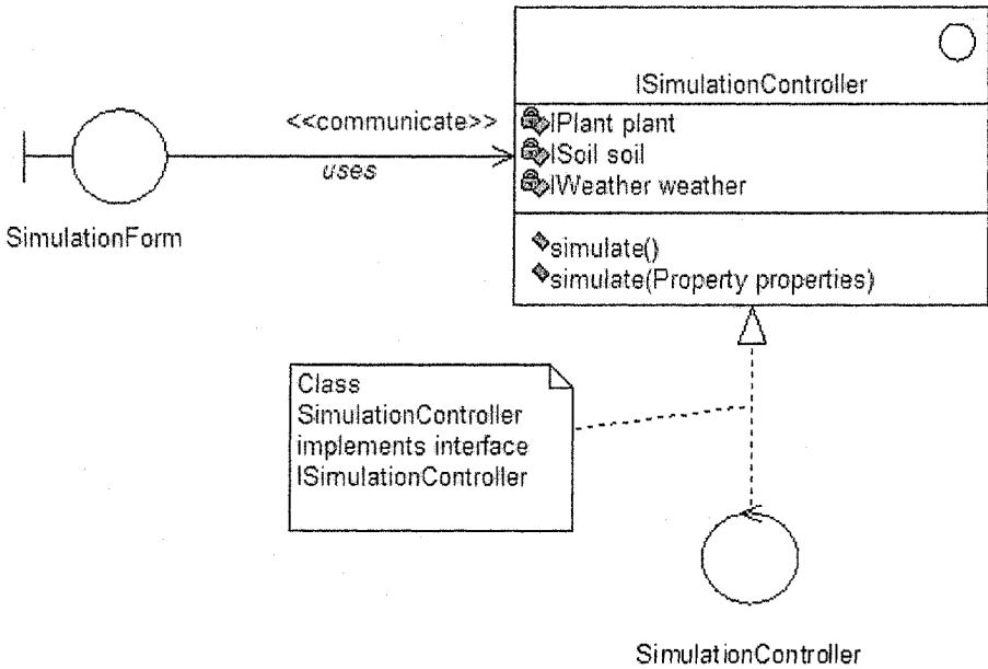
Figure 8-20. An interface defining the services of the control class SimulationController .
