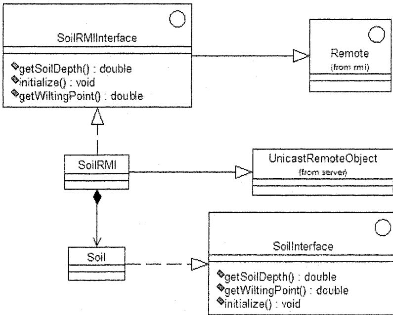
Figure 11-15. Class diagram for the implementation of SoilRMI server.
