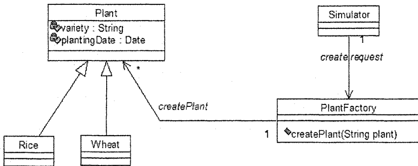
Figure 7-4. The factory method pattern.
