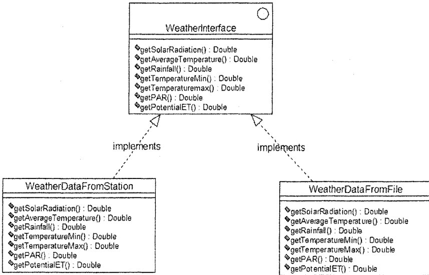
Figure 3-8. Example of two different classes implementing the same interface.
