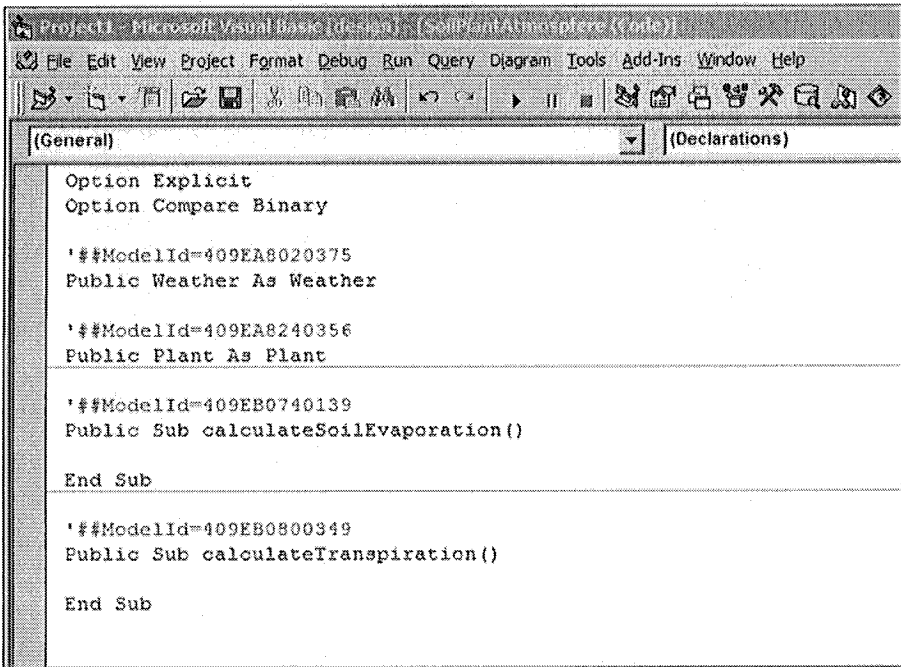
Figure 10-10. Example of code generation in Visual Basic for class SoilPlantAtmosphere.
