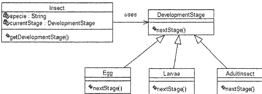
Figure 7-20. The UML diagram for the state pattern.
