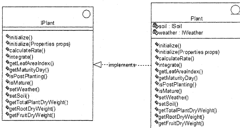
Figure 8-29. Class Plant implements the behavior defined in interface IPlant.
