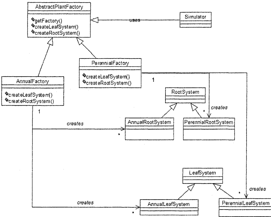
Figure 7-6. Class diagram of the abstract factory pattern.
