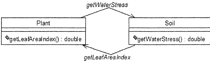
Figure 6-4. Interactions between Plant and Soil.
