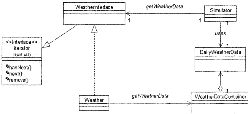
Figure 7-16. Classes involved in the iterator pattern.
