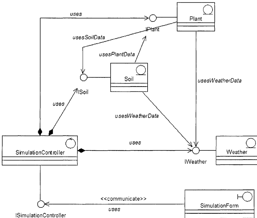
Figure 8-27. Final class diagram for the Kraalingen simulation approach.
