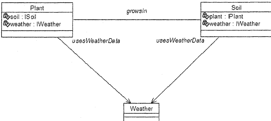
Figure 8-25. A monolithic system where entity classes are directly linked to each other.
