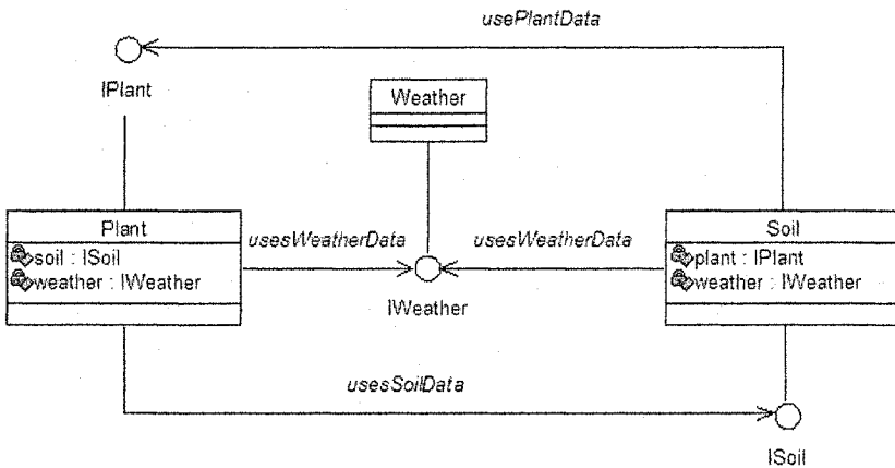
Figure 8-26. Classes have associations with an interface.
