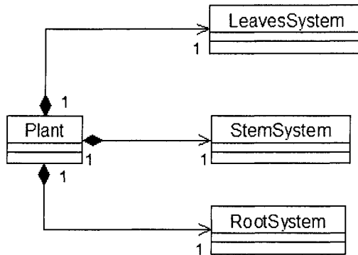
Figure 4-12. Plant is considered as a composition of its root, stem, and leaf systems.
