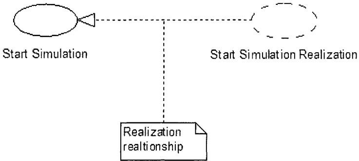
Figure 8-3. The use case realization for Start Simulation use case.
