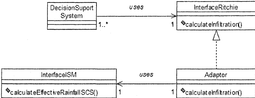
Figure 7-9. Class diagram for the adaptor pattern.
