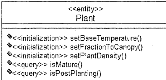
Figure 3-17. Using stereotypes to classify operations.
