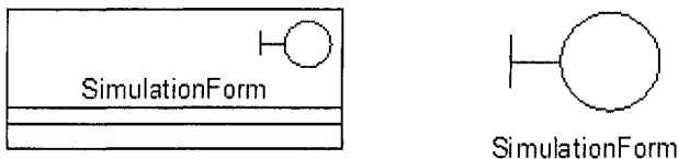
Figure 8-10. UML symbols for a boundary class.
