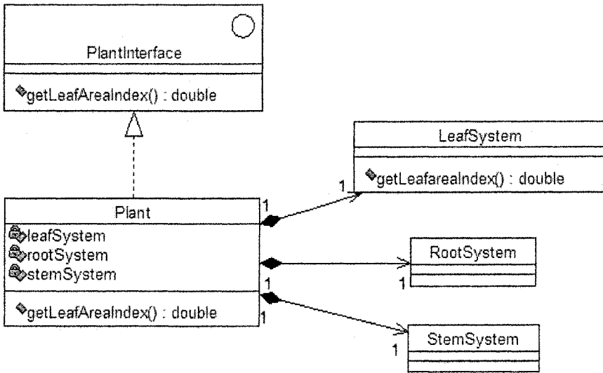
Figure 7-2. Example of delegation.
