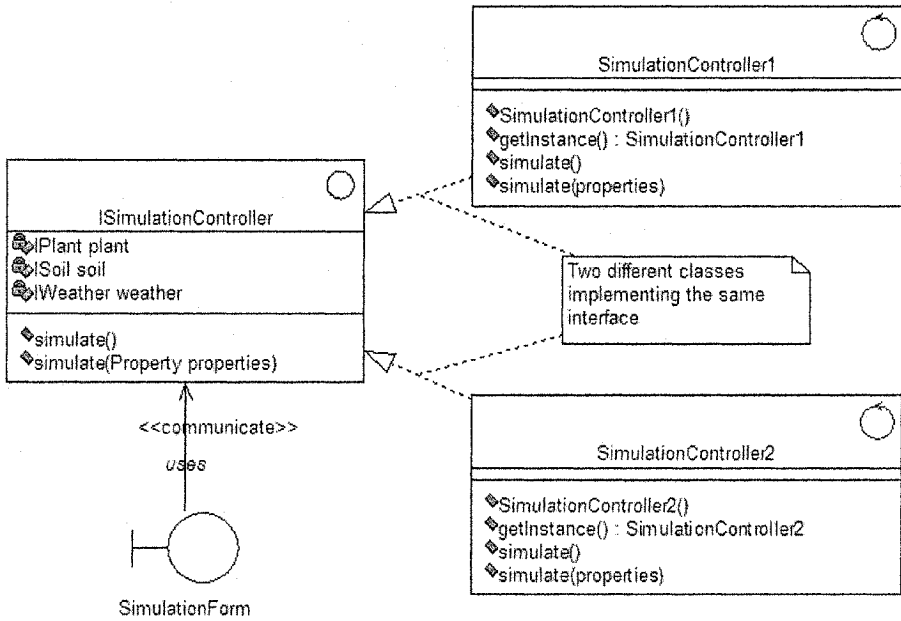
Figure 8-21. One boundary class associated with many control classes.
