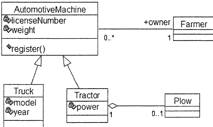
Figure 4-19. A subclass inherits from the superclass attributes, operations, and relationships.
