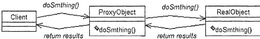
Figure 7-15. Communication between the proxy and the real object.
