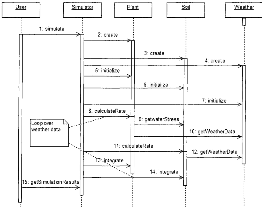
Figure 8-4. Sequence diagram for the Start Simulation use case.
