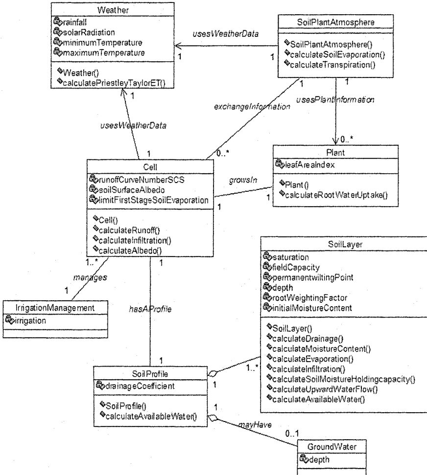
Figure 10-5. Class diagram for Ritchie's model.
