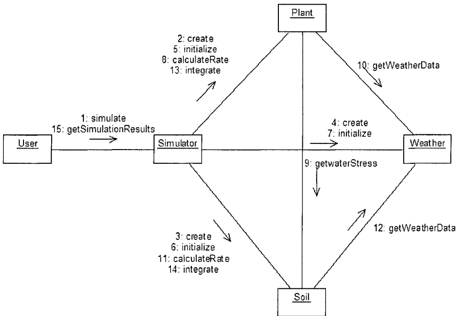
Figure 8-5. Collaboration diagram for the use case Start Simulation.
