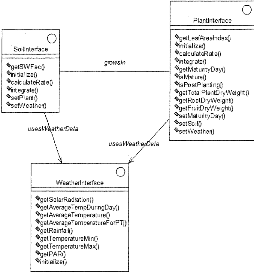
Figure 11-18. Conceptual diagram for the Kraalingen crop simulation model.
