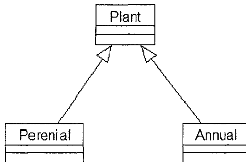
Figure 4-16. UML notation for the relationship of generalization.
