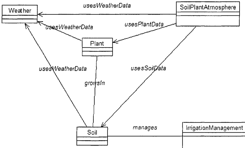
Figure 10-3. Conceptual model that considers soil-plant-atmosphere processes.
