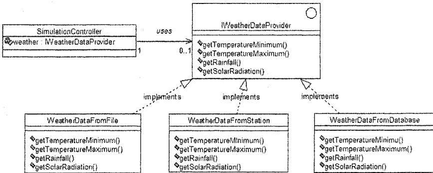
Figure 9-1. Strategy pattern used for implementing a plug and play architecture.
