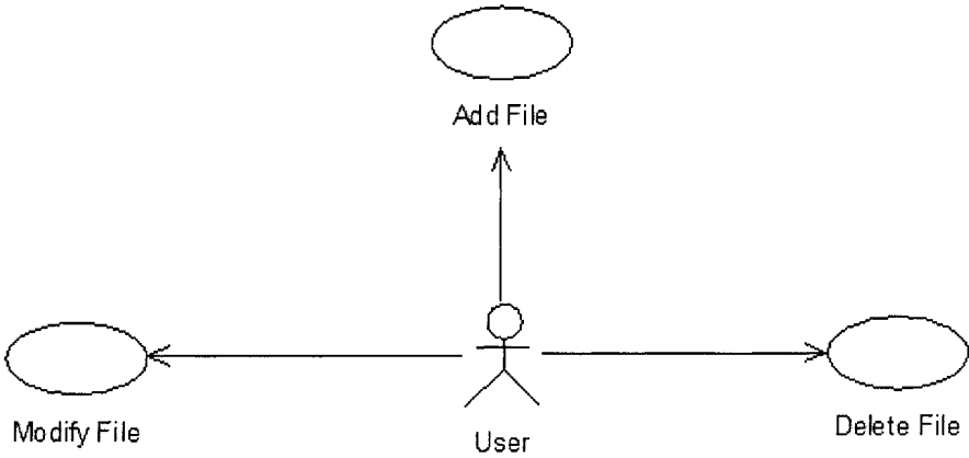
Figure 6-2. Example of bad selection of use cases.
