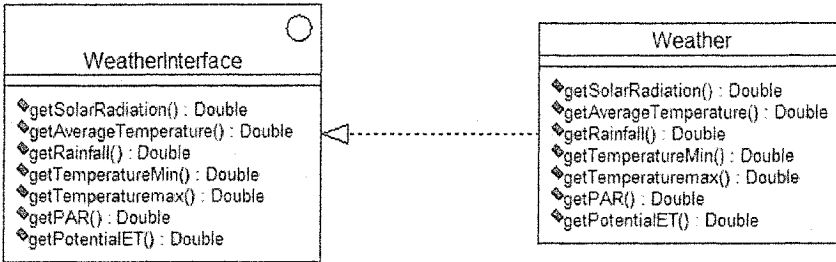
Figure 3-6. Class implementing an interface.
