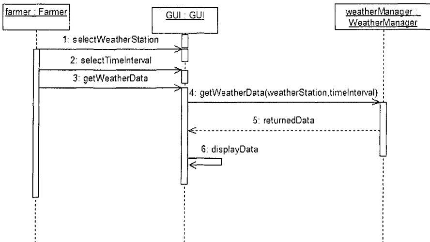
Figure 6-5. Example of a sequence diagram.
