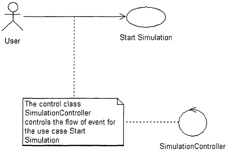
Figure 8-13. SimulationController controls the flow of events for the use case.
