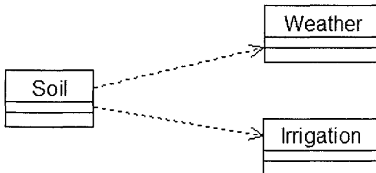
Figure 4-15. One class depends on two other classes.
