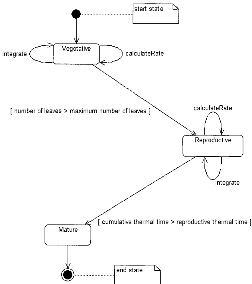
Figure 6-12. States of object plant during the simulation.
