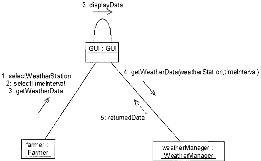
Figure 6-9. Example of a collaboration diagram.
