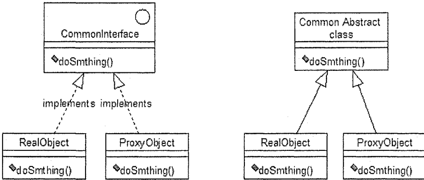
Figure 7-14. Class diagram for the proxy object.
