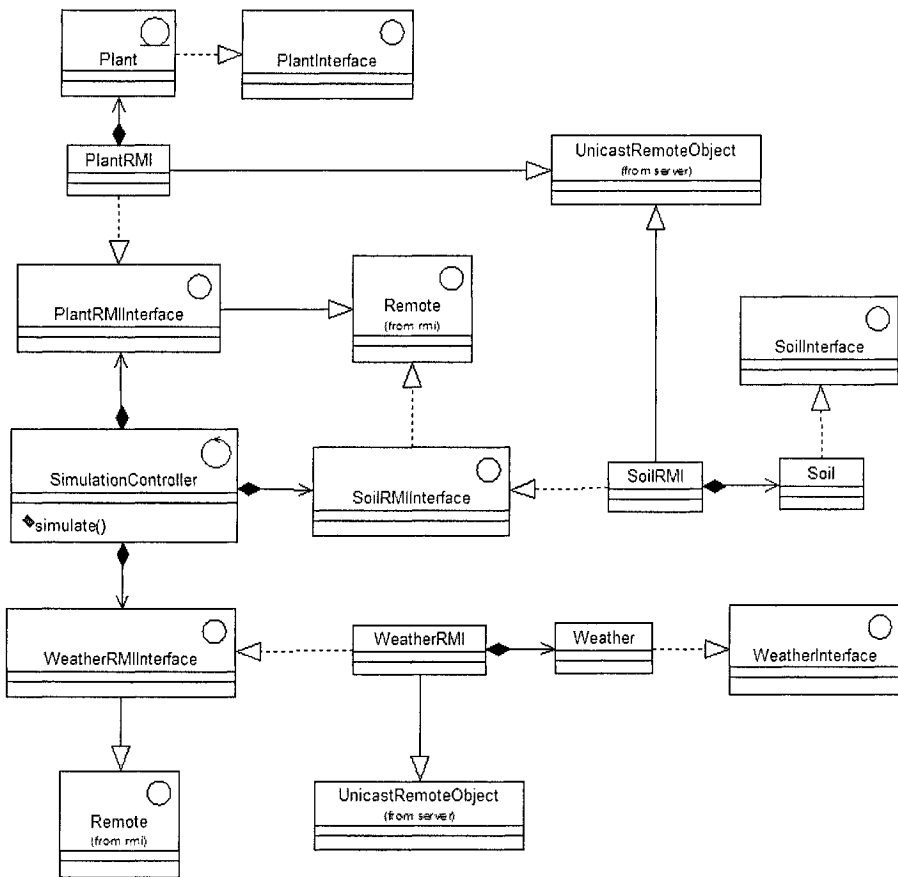
Figure 11-20. Class diagram for Kraalingen distributed system.
