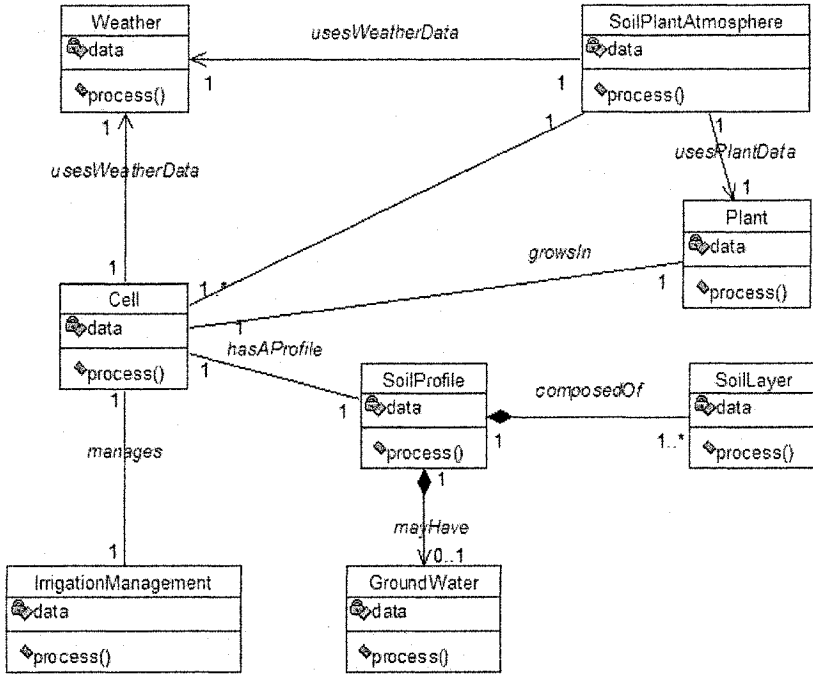
Figure 10-4. Template for developing new water-balance or irrigation-scheduling models.
