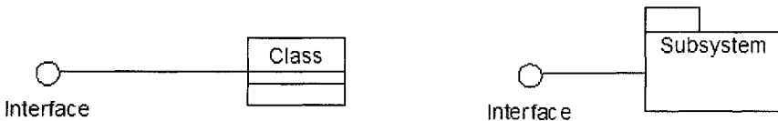
Figure 4-22. Examples of realizations.
