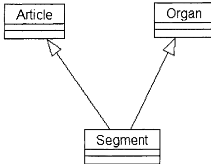
Figure 4-20. Class Segment inherits from both classes Article and Organ.
