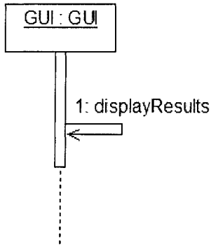
Figure 6-8. Example of a reflexive message.
