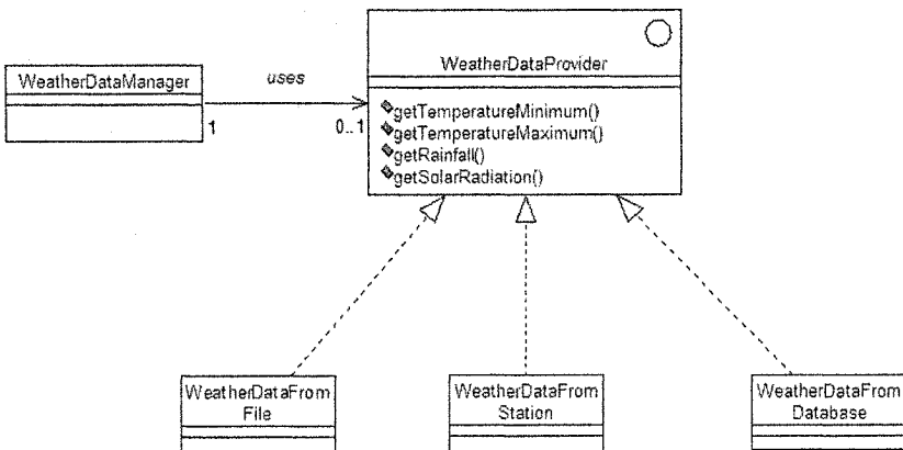
Figure 7-21. Class diagram for the strategy pattern.
