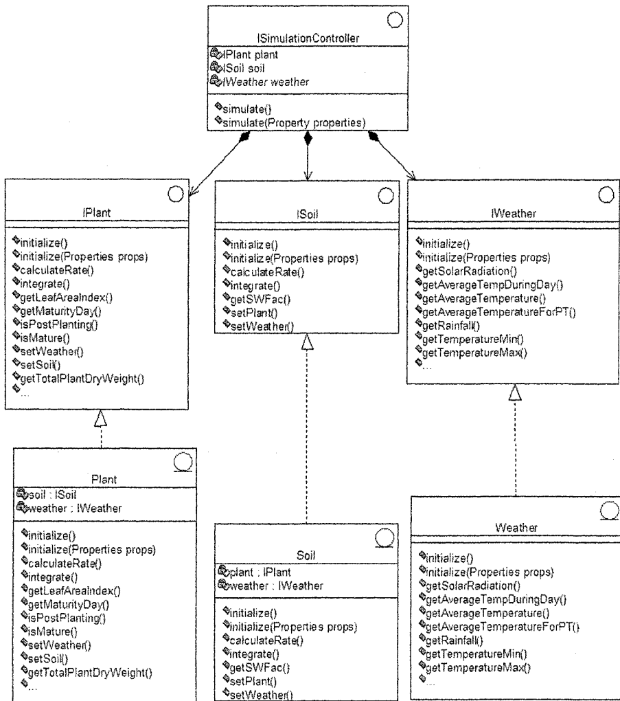
Figure 8-23. The control object communicates with entity objects through interfaces.
