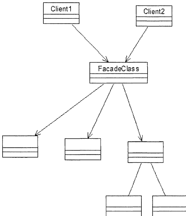
Figure 7-18. Class diagram for the facade pattern.
