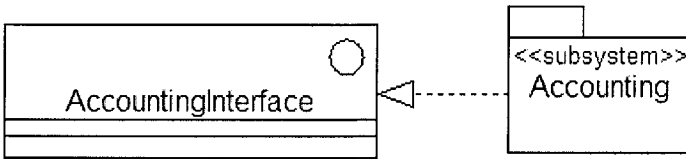
Figure 3-12. Example of UML symbol of a subsystem.
