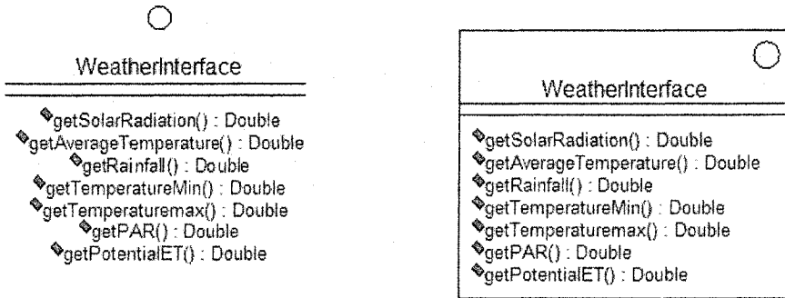
Figure 3-4. UML symbols for an interface.
