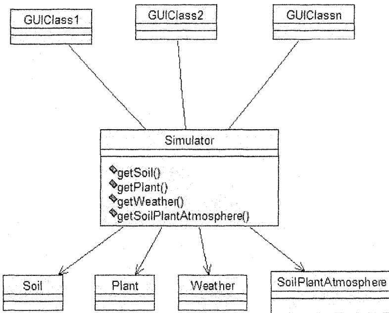
Figure 7-19. Communication with GUI classes goes through the Simulator.
