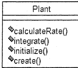
Figure 8-7. The definition of behavior for class Plant.
