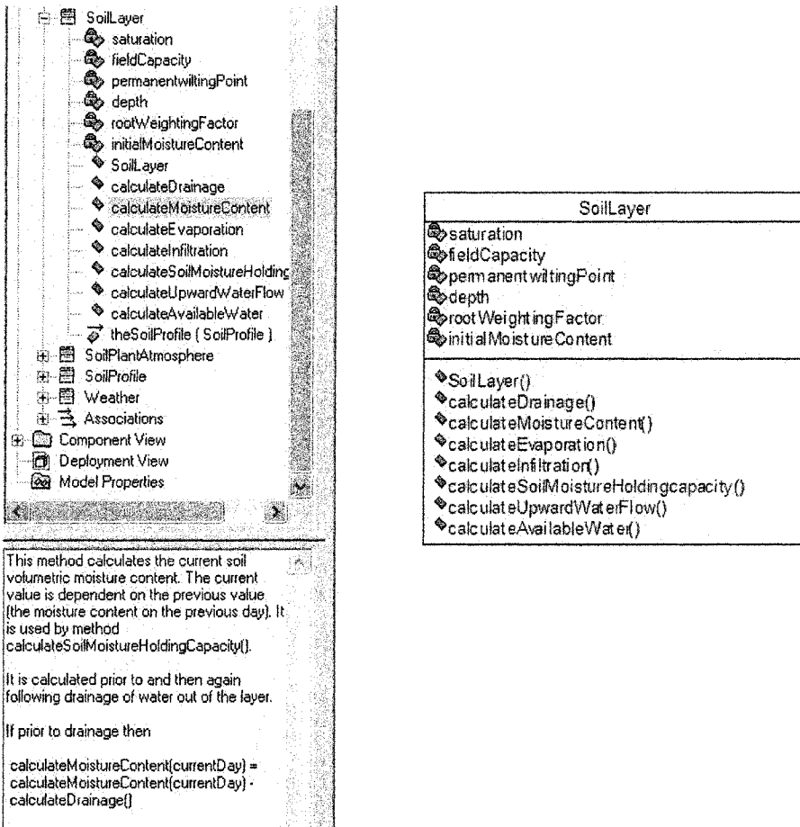
Figure 10-7. Example of documentation provided for a method.
