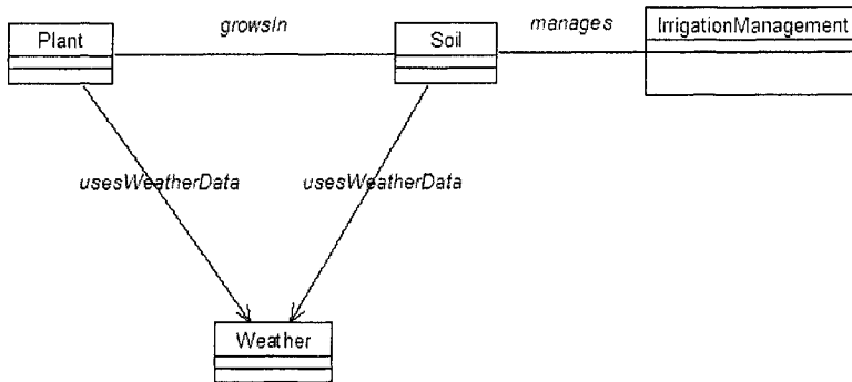
Figure 10-2. Conceptual model with irrigation management considerations.
